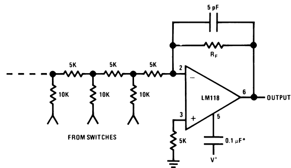
D/A Converter Using Ladder Network
