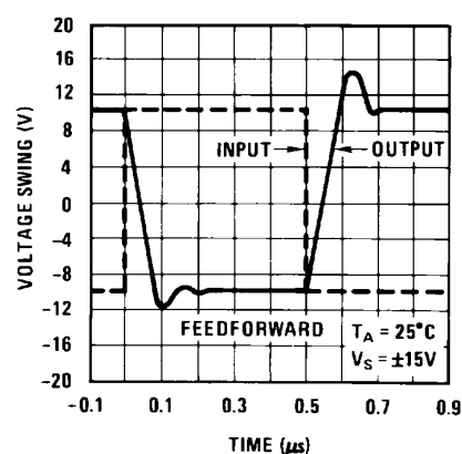
Inverter Pulse Response
