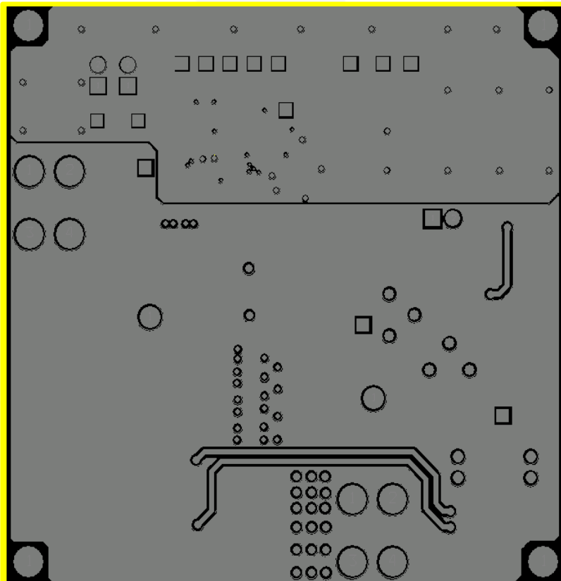
Figure 31. Evaluation Board Inner Layer 1 Copper
