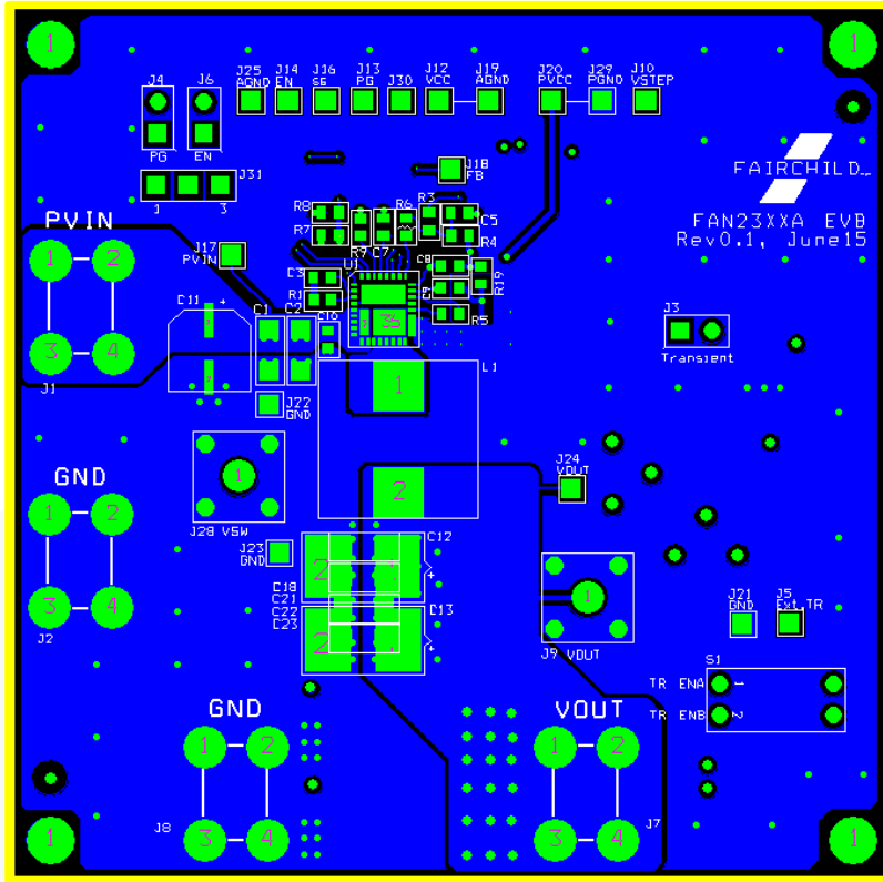
Figure 30. Evaluation Board Top Layer Copper
