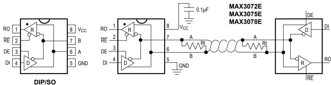
TYPICAL HALF-DUPLEX OPERATING CIRCUIT
