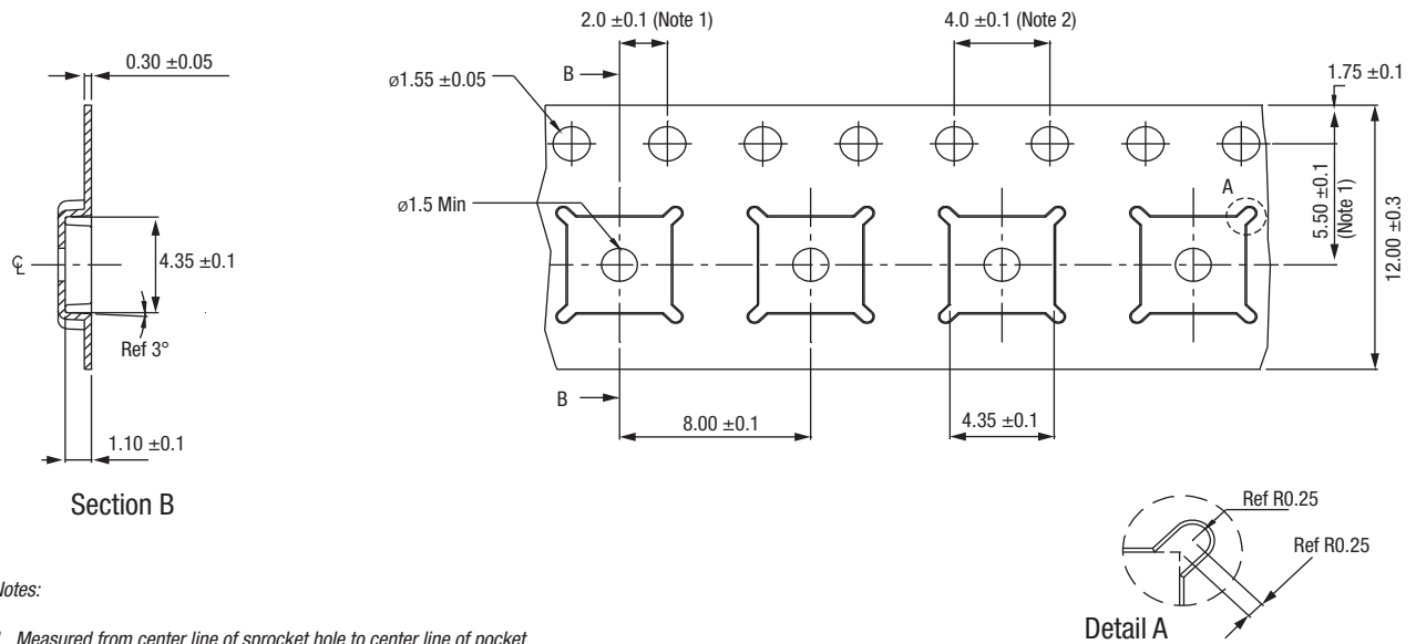
Figure 15. SKY85402-11 20-Pin QFN Tape and Reel Dimensions
