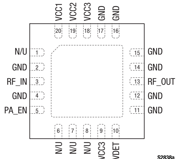
Figure 1. SKY85402-11 Pinout – 20-Pin QFN (Top View)
