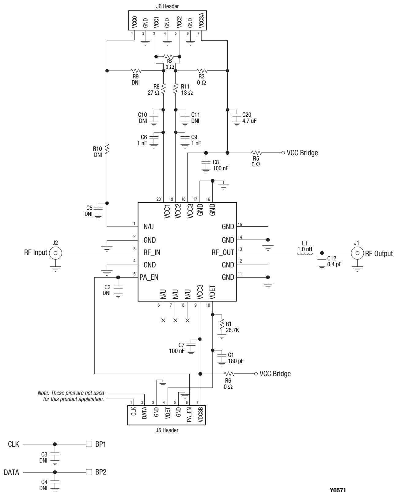
Figure 10. SKY85402-11 Evaluation Board Schematic
