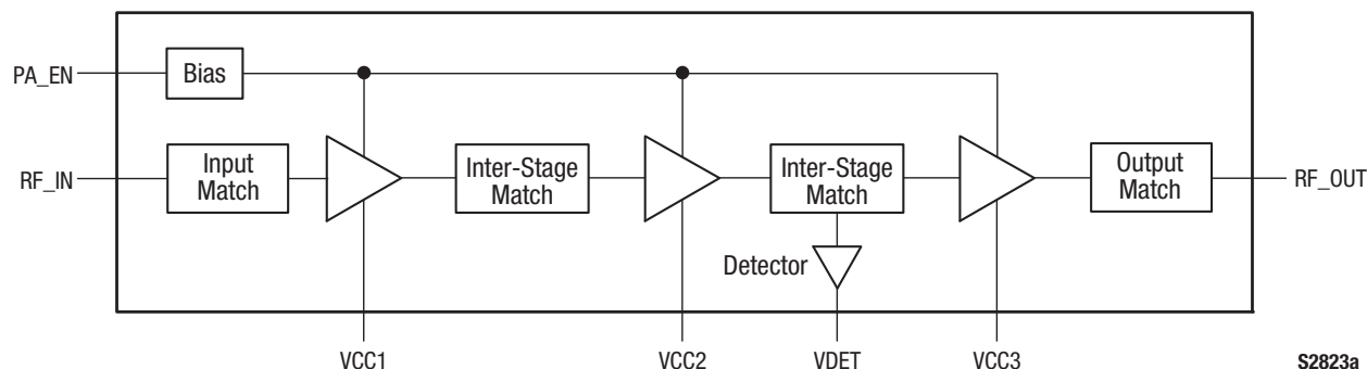
Figure 2. SKY85402-11 Block Diagram
