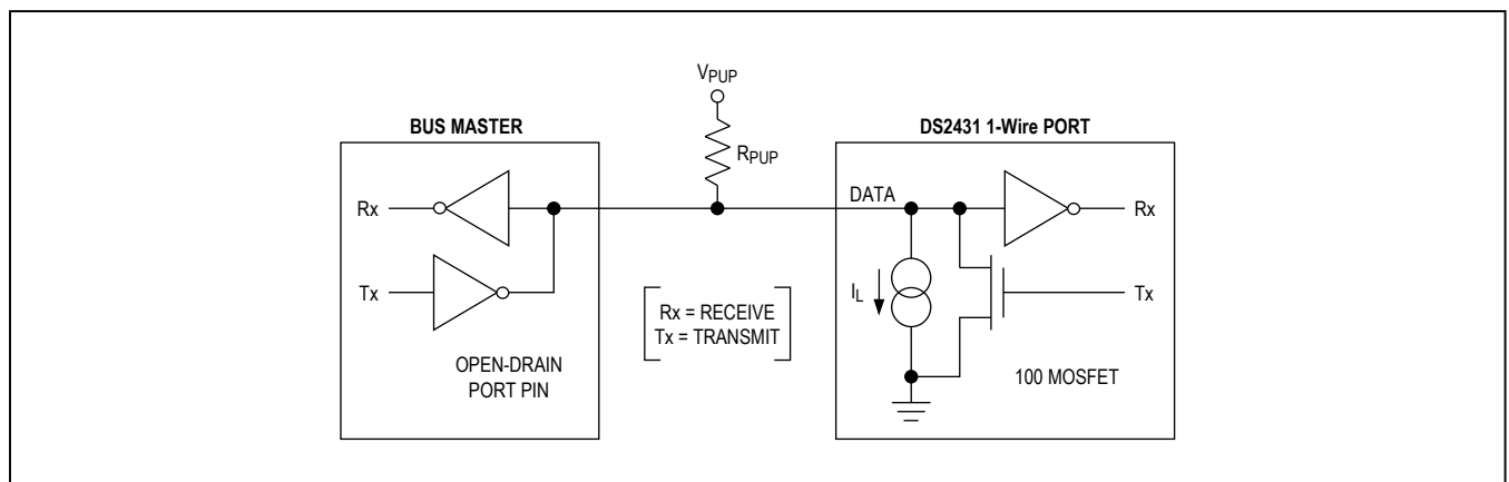
Figure 8. Hardware Configuration
