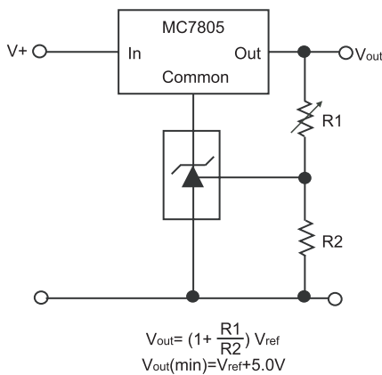
Figure 23. Output Control for a Three-Terminal Fixed Regulator
