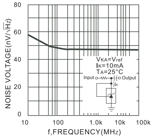
Figure 16. Spectral Noise Density
