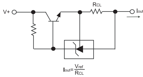
Figure 25. Constant Current Source
