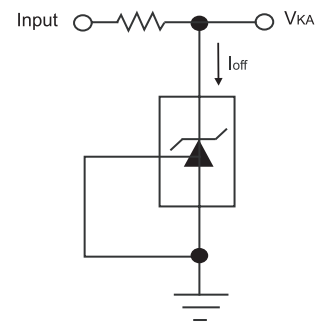
Figure 6. Test Circuit for I_{off}
