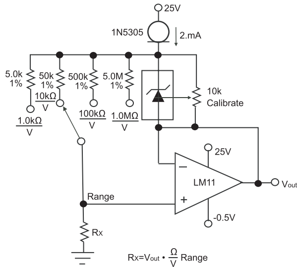
Figure 31. Linear Ohmmeter
