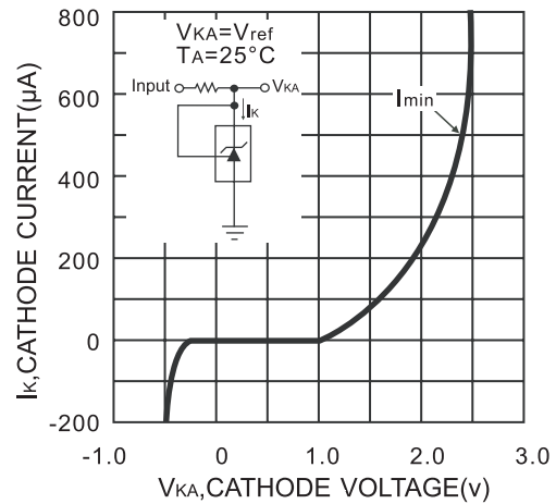
Figure 8. Cathode Current vs. Cathode Voltage
