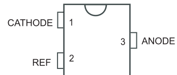
TL431, A, B DBZ (SOT-23)PACKAGE (Top View)
