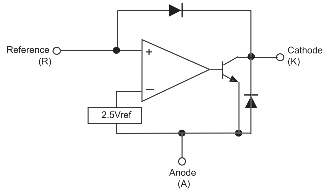
Figure 2. Block Diagram
