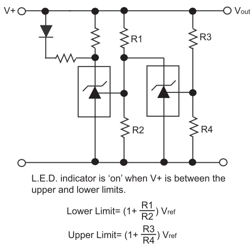
Figure 29. Voltage Monitor
