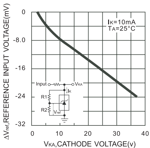
Figure 11. Change in Reference Input Voltage vs. Cathode Voltage
