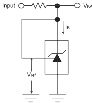
Figure 4. Test Circuit for V_{KA}=V_{REF}
