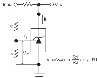
Figure 5. Test Circuit for V_{KA} \geq V_{REF}
