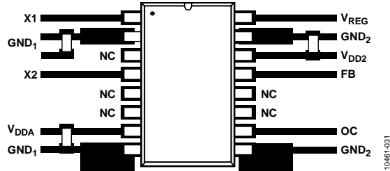
Figure 34. Recommended PCB Layout
