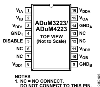
Figure 4. Pin Configuration
