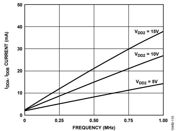
Figure 10. Typical I_{DD1} , I_{DD2} Supply Current vs. Frequency with 2 nF Load
