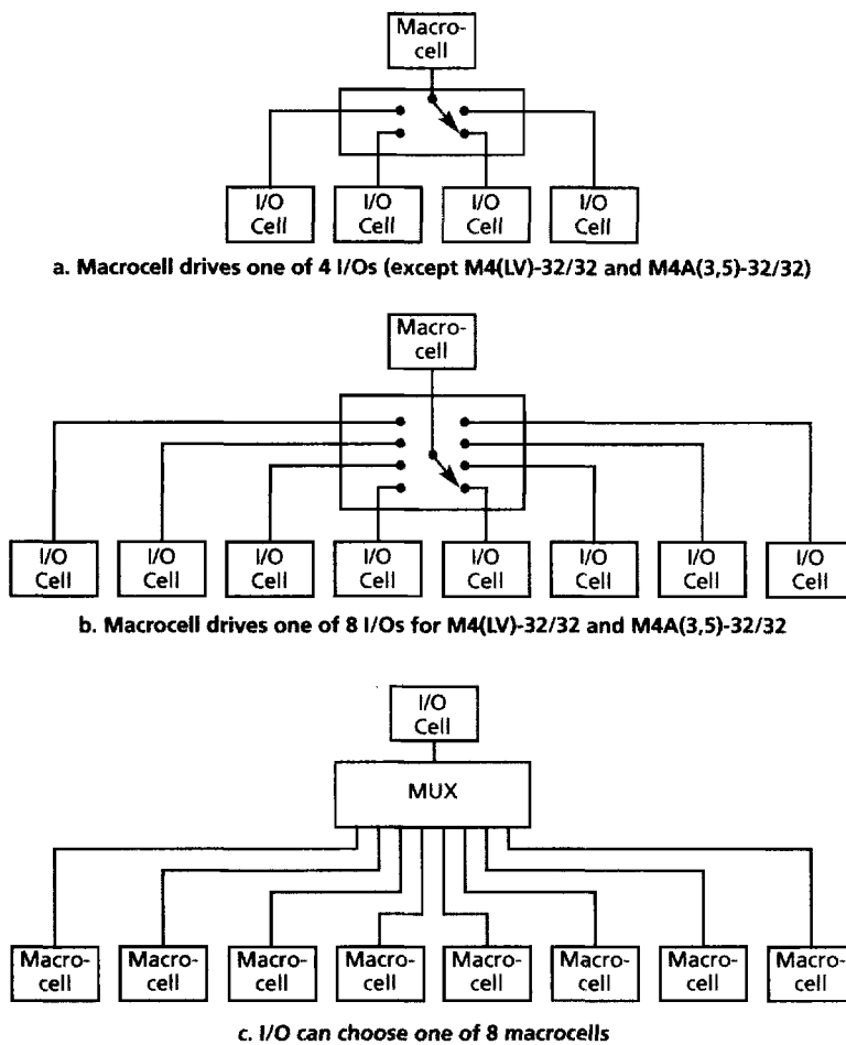
Figure 9. MACH 4 Output Switch Matrix
