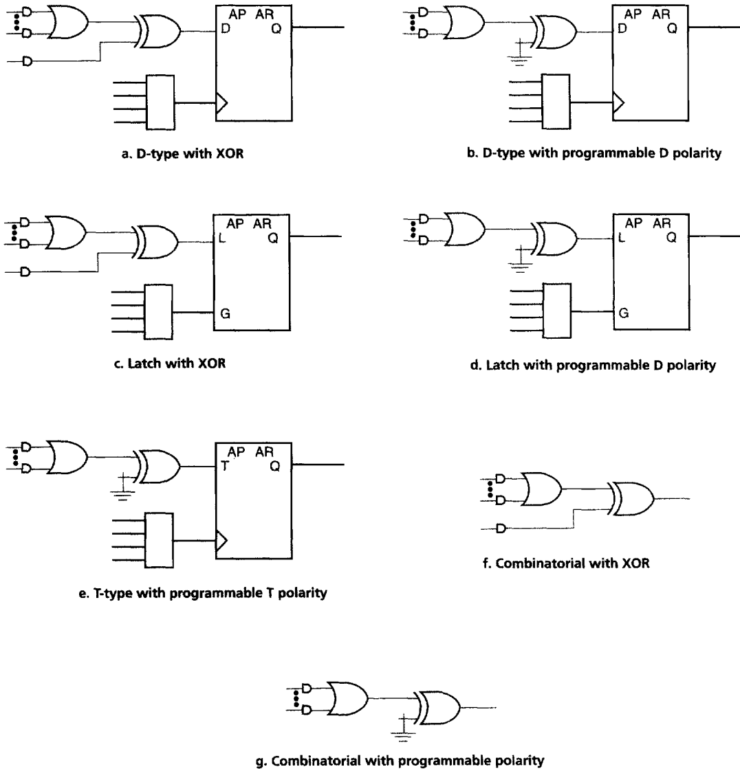
Figure 6. Primary Macrocell Configurations
