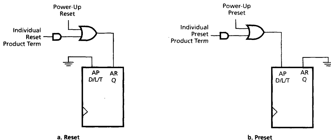
Figure 8. Asynchronous Mode Initialization Configurations
