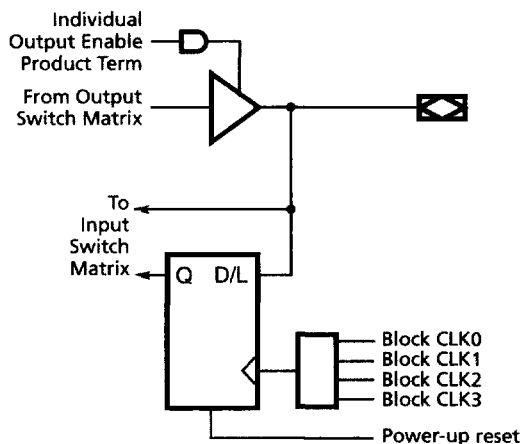
Figure 10. I/O Cell for MACH 4 Devices (except M4(LV)-32/32 and M4A(3,5)-32/32)
