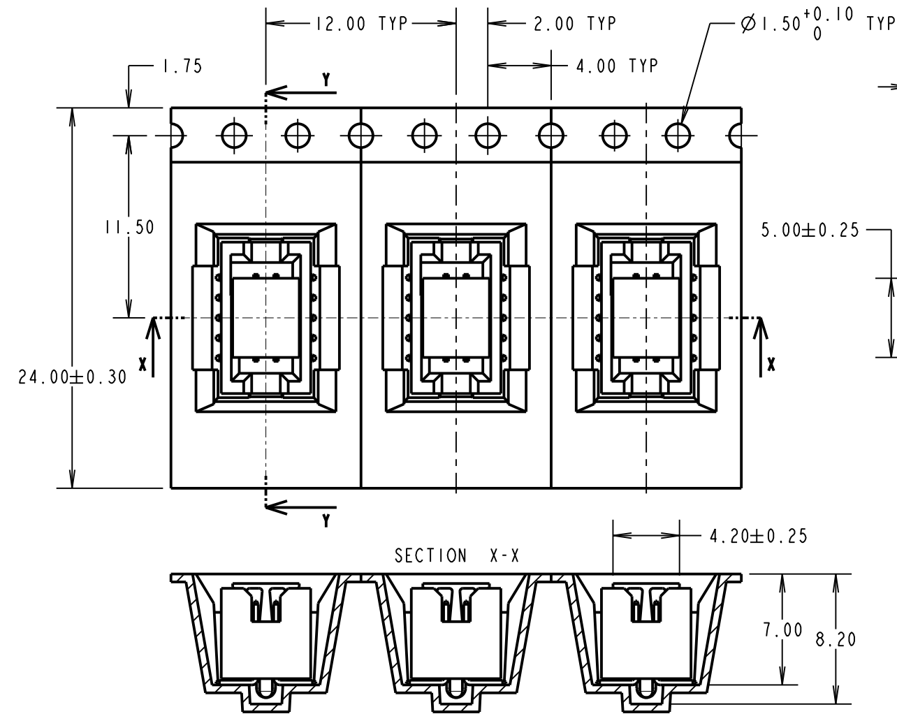
TAPE DETAILS FOR 05 WAY ONLY
