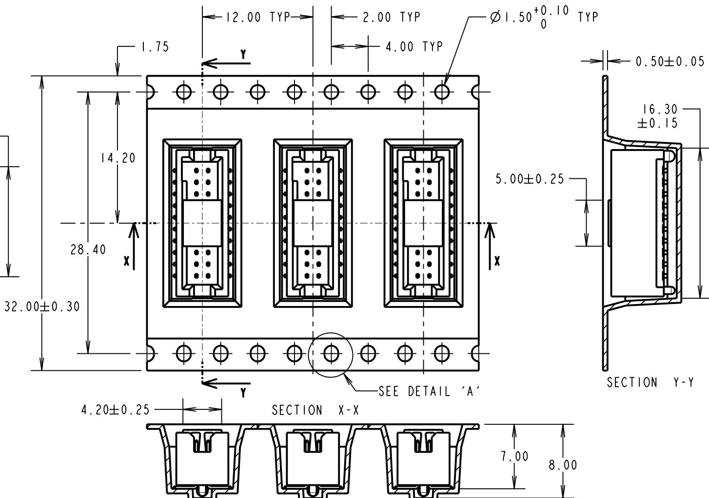
TAPE DETAILS FOR 10 WAY ONLY
