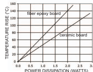
POWER DERATING
