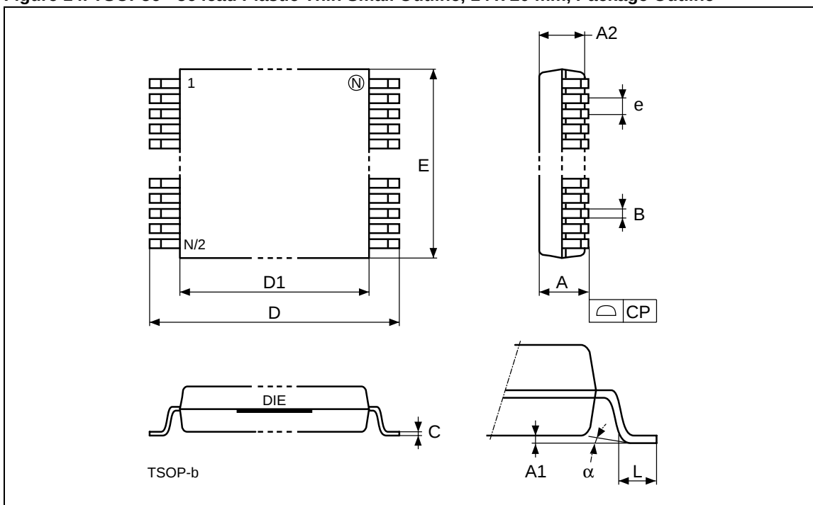
Figure 14. TSOP56 - 56 lead Plastic Thin Small Outline, 14 x 20 mm, Package Outline
