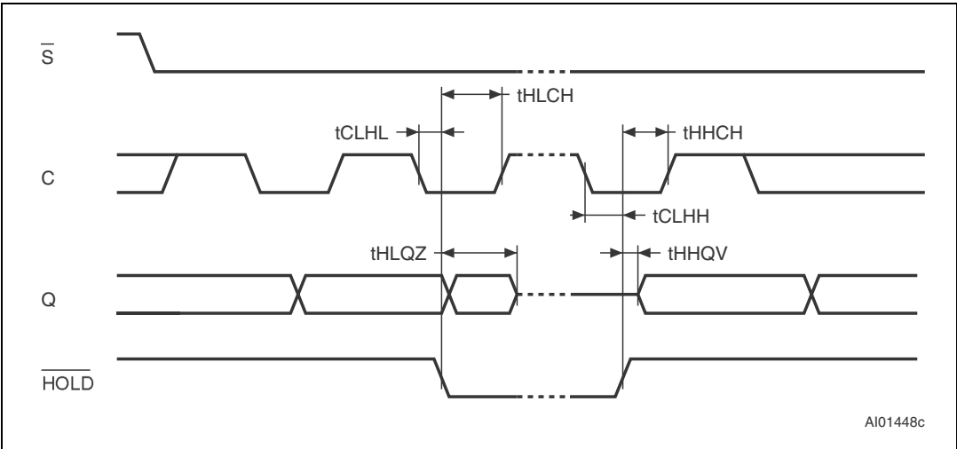
Figure 20. Hold timing
