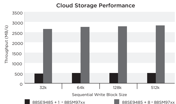
Fig 5. Sequential Write Performance
