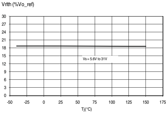
Figure 15. V_{Rlth} vs. T_j
