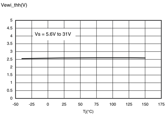
Figure 16. V_{EWi\_thh} vs. T_j
