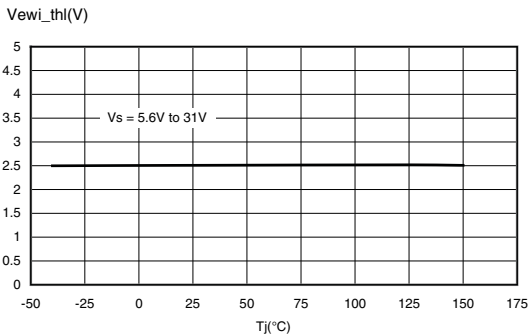
Figure 17. V_{EWi\_thl} vs. T_j
