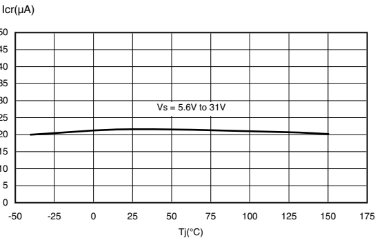
Figure 18. I_{cr} vs. T_j
