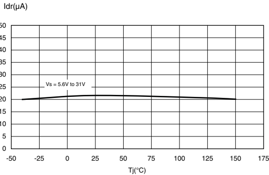
Figure 19. I_{dr} vs. T_j
