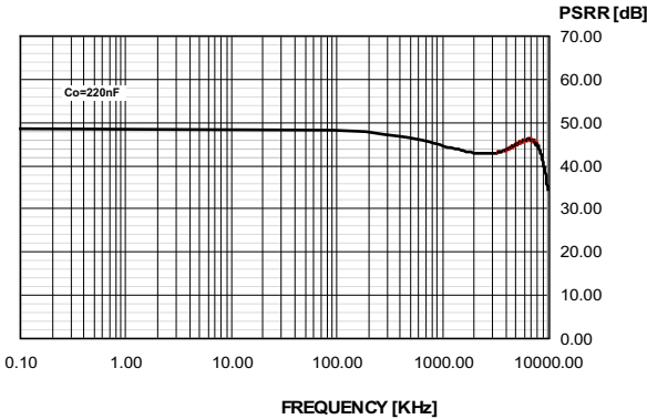
Figure 20. PSRR
