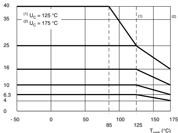
Fig. 5 - Maximum permissible voltage up to T_{amb} = 175^\circ\text{C}
