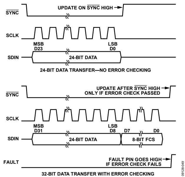
Figure 41. PEC Timing
