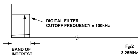
c) Use of Digital Filtering to Remove the Out-of-Band Quantization Noise
