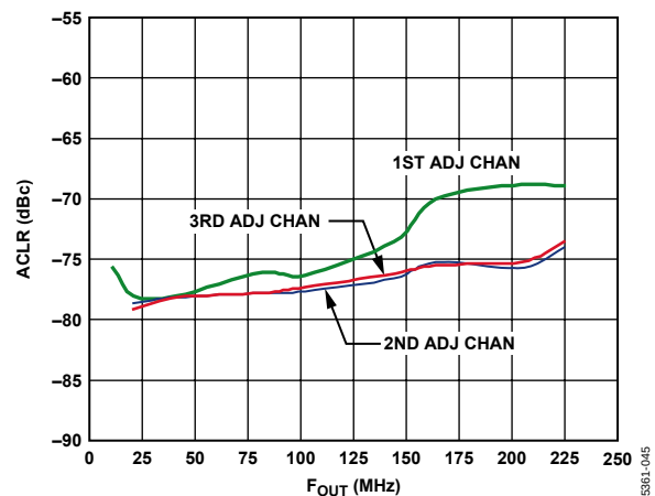
Figure 48. AD9776 ACLR, f_{\text{DATA}} = 122.88 \text{ MSPS} , 4x Interpolation, f_{\text{DAC}}/4 Modulation
