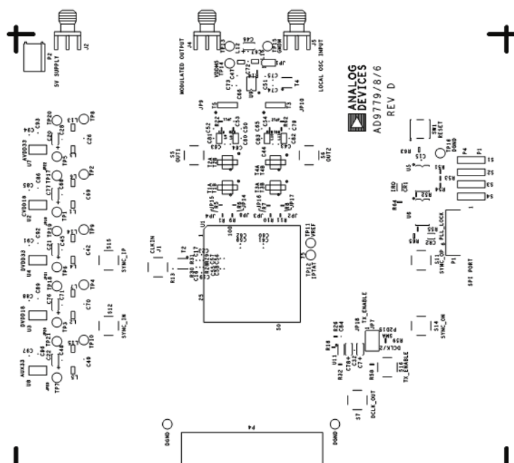
Figure 110. Evaluation Board, Rev. D, Top Silk Screen
