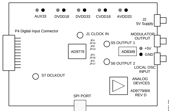
Figure 100. Typical Test Setup
