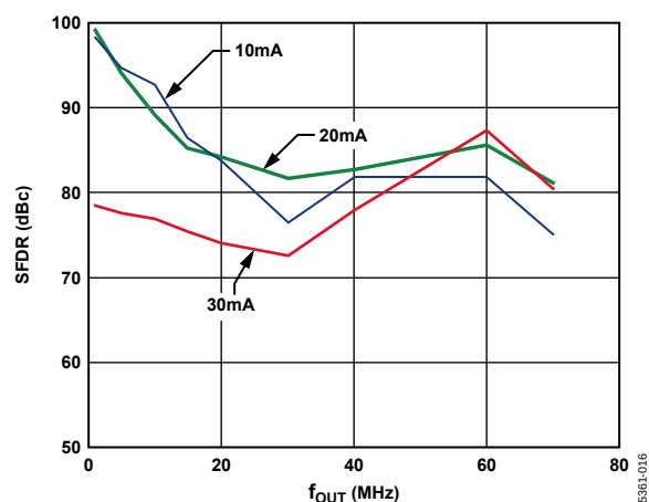
Figure 17. AD9779 In-Band SFDR vs. Output Full-Scale Current
