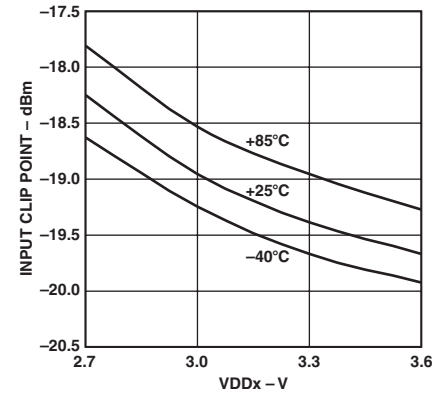
TPC 4c. Maximum VGA Attenuation Clip Point vs. Supply (Low Bias 3 )
