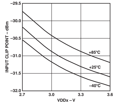
TPC 5c. Minimum VGA Attenuation Clip Point vs. Supply (Low Bias 3 )
