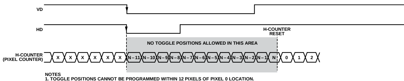
Figure 50. No-Toggle Positions
