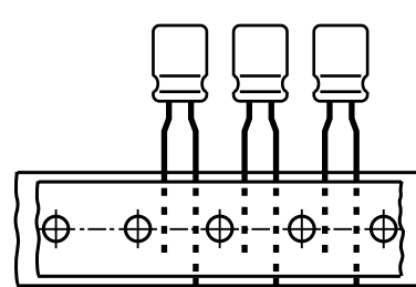
Case Ø D = 5 mm to 8 mm; Lead space F is 5 mm
