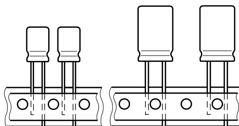
Dimensions of lead space F see table 2
