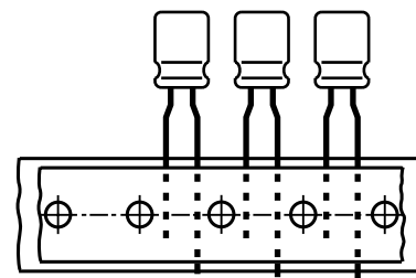
Case Ø D = 5 mm to 8 mm; Lead space F is 5 mm
