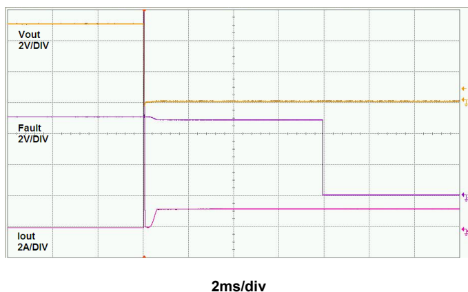
Figure 7 Short-Circuit Current Limit Response
