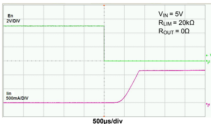
Figure 5 Device Enabled into Short-circuit
