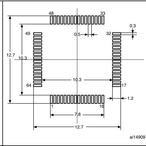
Figure 72. Recommended footprint (1)(2)
