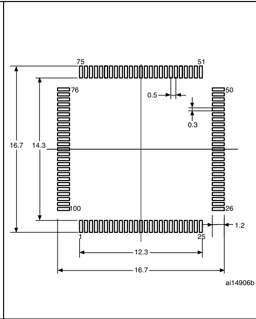
Figure 70. Recommended footprint (1)(2)
