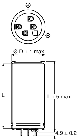
Fig. 8 - Printed wiring pin version (case Ø D = 40 mm)
