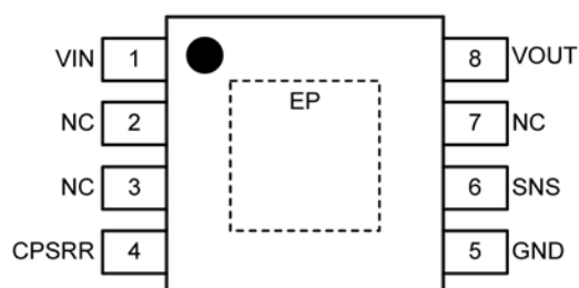
8-Pin ePad MSOP MAQ5282-x.xYMME
