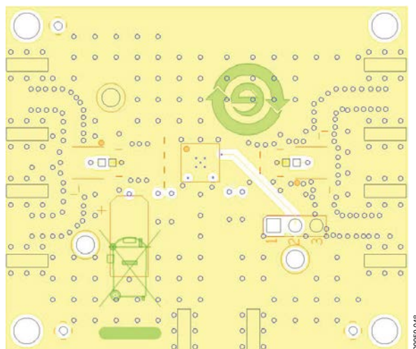
Figure 47. Layout of Evaluation Board, Circuit Side
