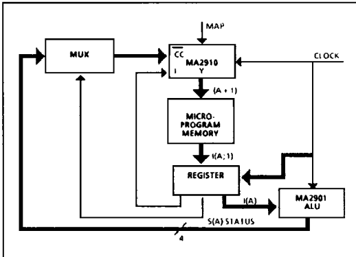
Figure 20: Instruction Based
