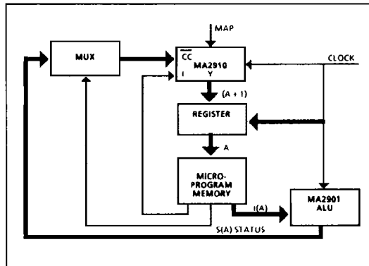
Figure 22: Address Based
