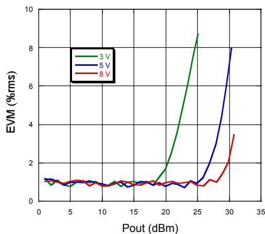
EVM vs. Pout
