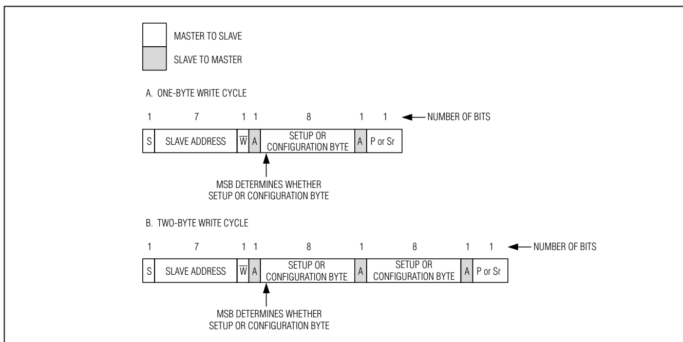
Figure 9. Write Cycle
