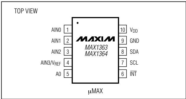
Pin Configuration
