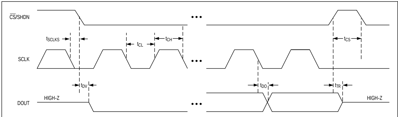
Figure 7. Detailed Serial-Interface Timing Sequence
