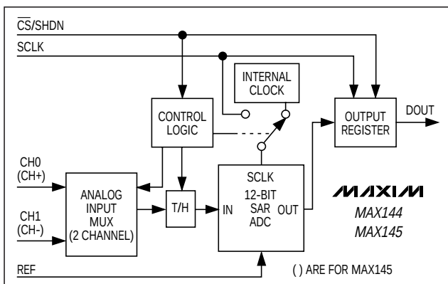
Figure 2. Simplified Functional Diagram
