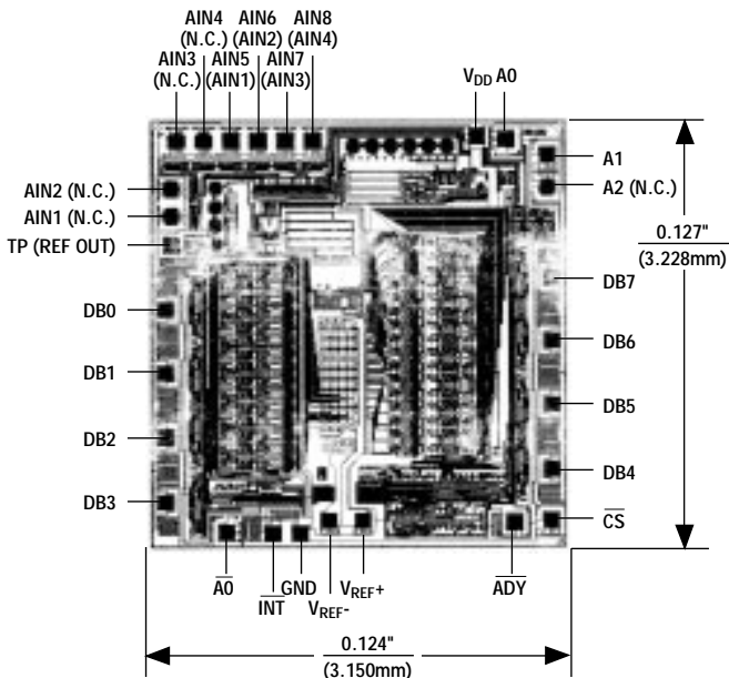
Chip Topography
