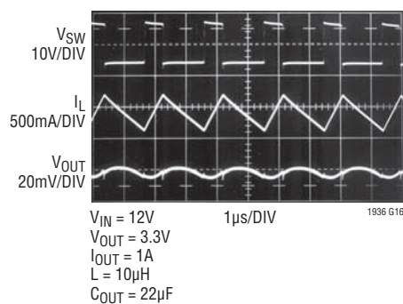
Switching Waveforms
