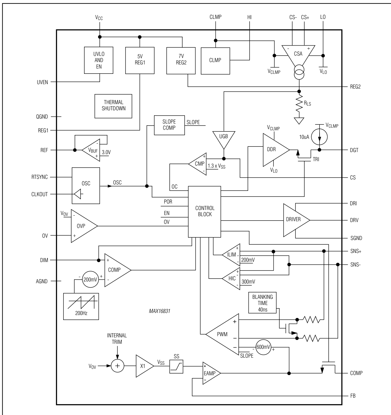
Functional Diagram
