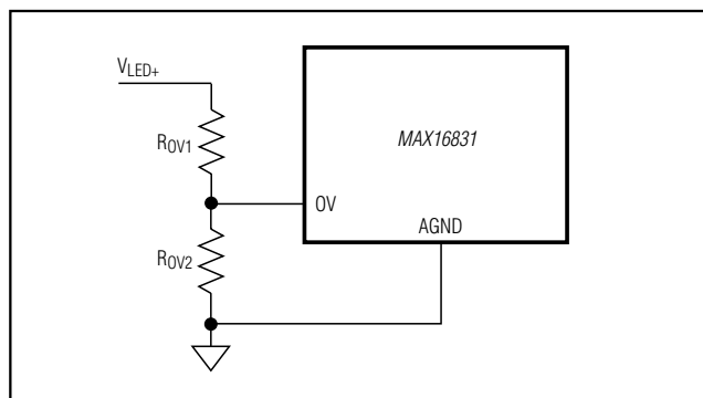
Figure 4. Setting the Overvoltage Threshold
