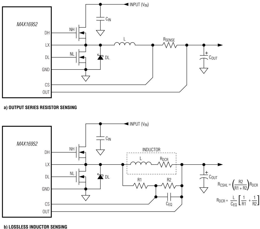
Figure 4. Current-Sense Configurations
