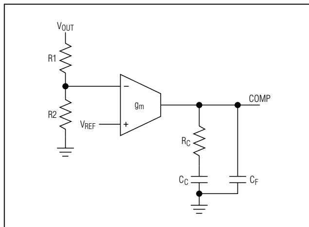
Figure 5. Compensation Network
