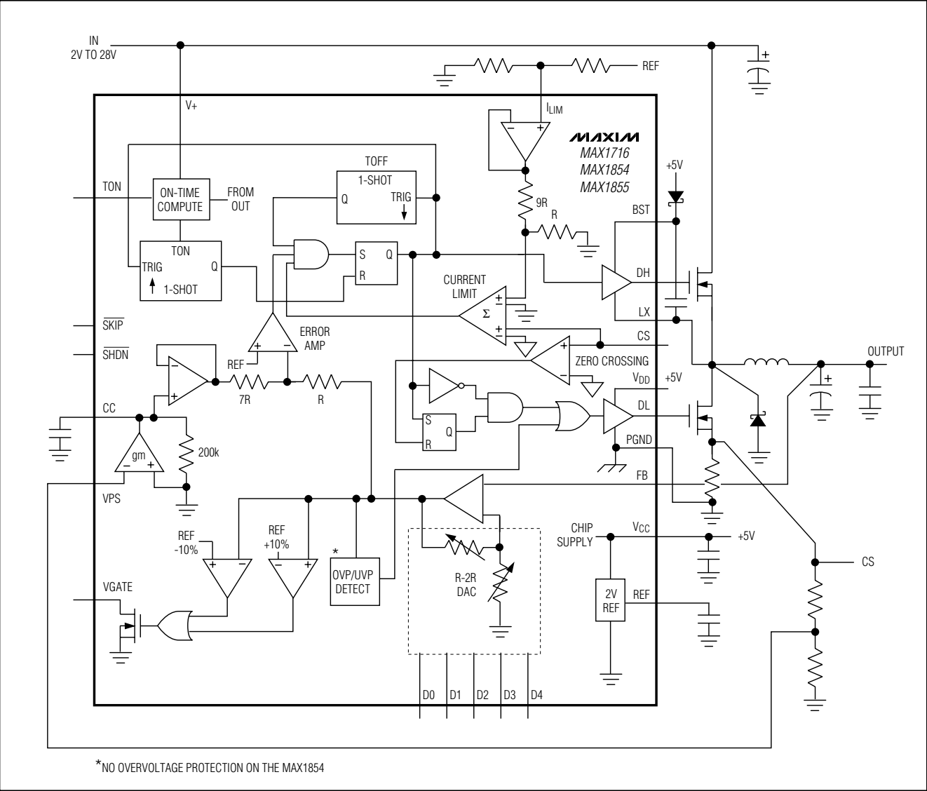
Figure 2. Functional Diagram
