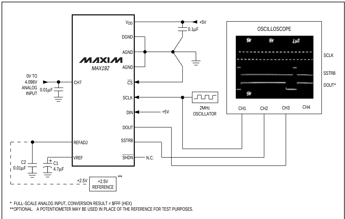
Figure 5. Quick-Look Circuit
