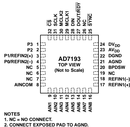
Figure 6. 32-Lead LFCSP Pin Configuration
