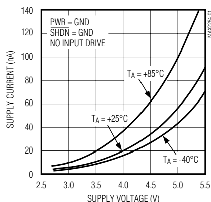
MAX2264 SHUTDOWN CURRENT vs. SUPPLY VOLTAGE
