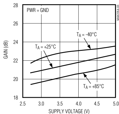
MAX2264 GAIN vs. SUPPLY VOLTAGE
