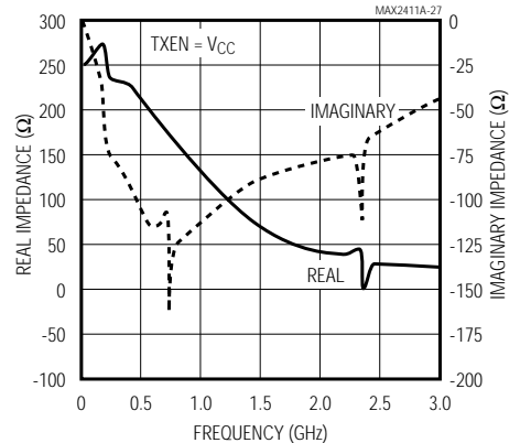
TRANSMIT MIXER OUTPUT IMPEDANCE vs. FREQUENCY
