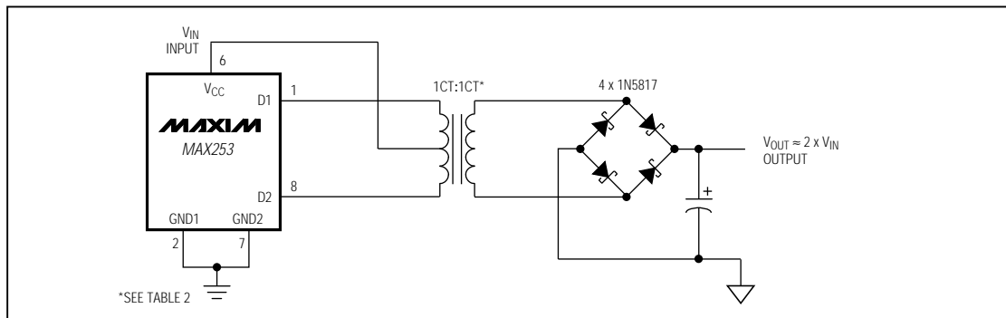
Figure 9c. Full-Wave Rectifier—Unipolar
