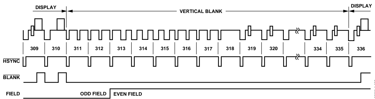
Figure 25. Timing Mode 1 (PAL)
