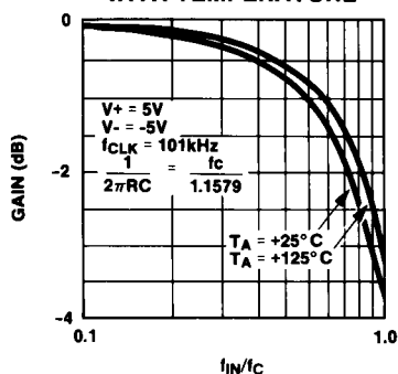
VARIATION OF PASSBAND GAIN WITH TEMPERATURE
