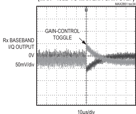
Rx BASEBAND DC OFFSET SETTLING RESPONSE WITH RxHP = 0 (MAX - 40dB TO MAX LNA GAIN STEP)
