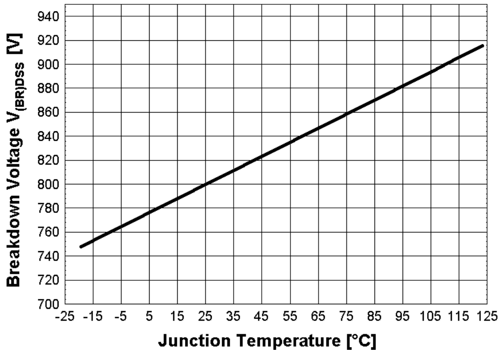
Figure 9 Drain-source breakdown voltage; V_{BR(DSS)} = f(T_J) , I_D = 0.25\text{mA}
