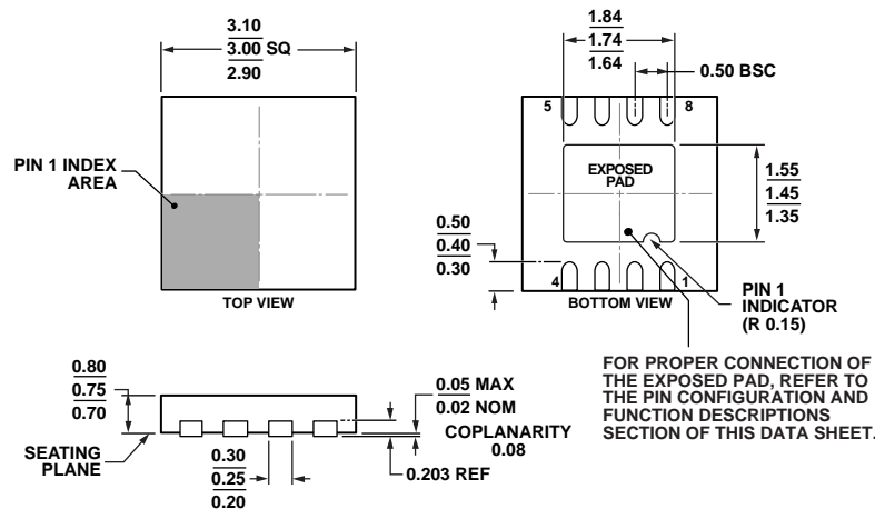
Figure 73. 8-Lead Lead Frame Chip Scale Package [LFCSF_WD] 3 mm × 3 mm Body, Very Very Thin, Dual Lead (CP-8-13)
