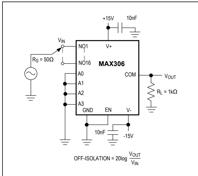
Figure 6. Off-Isolation
