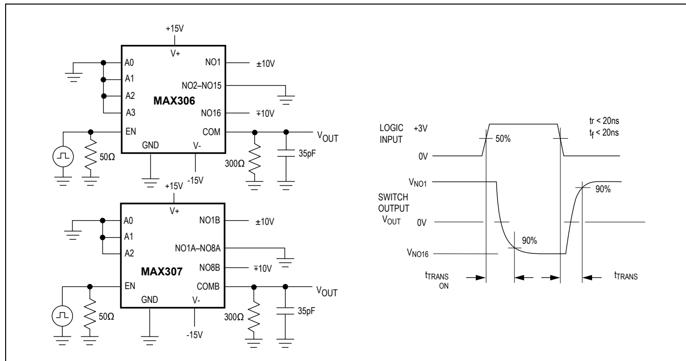
Figure 2. Transition Time
