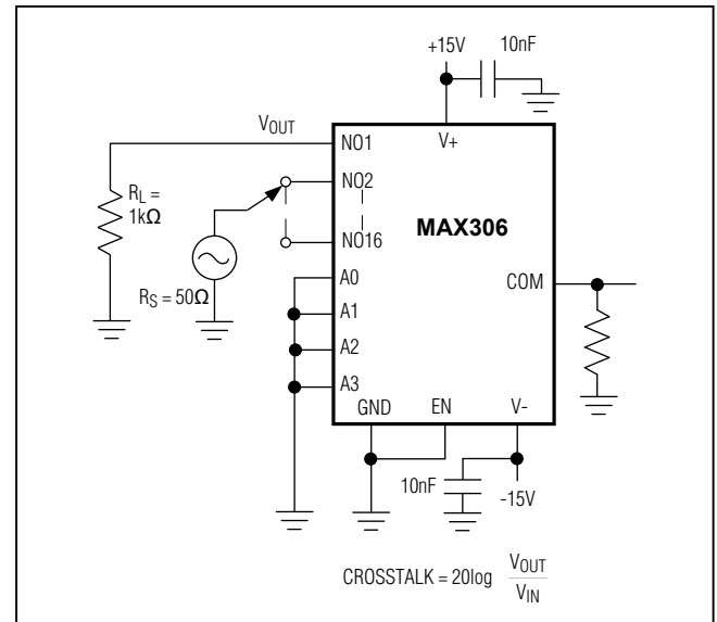
Figure 7. Crosstalk
