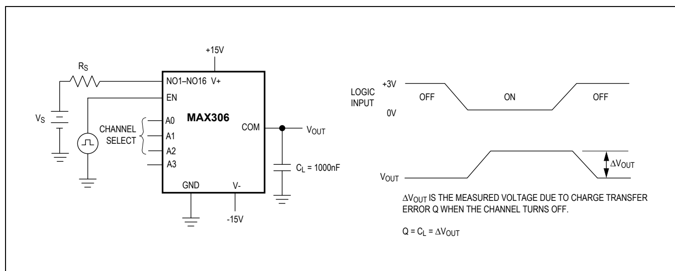
Figure 5. Charge Injection
