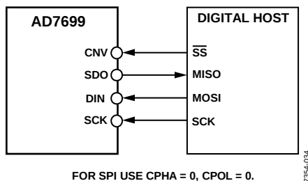
Figure 39. Connection Diagram for the AD7699 Without a Busy Indicator
